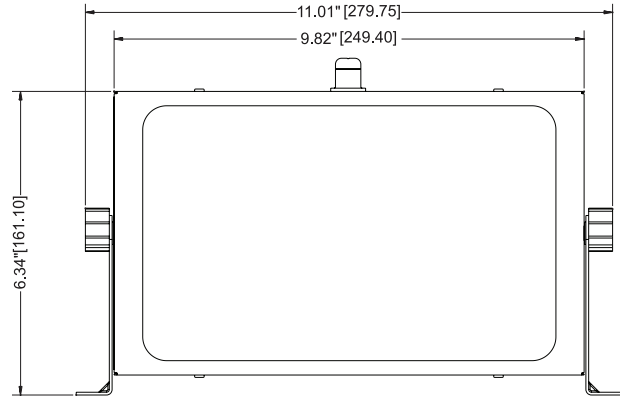
Bottom Mount
