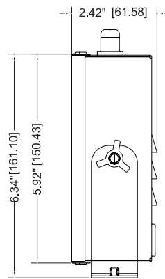
Bottom Mount
