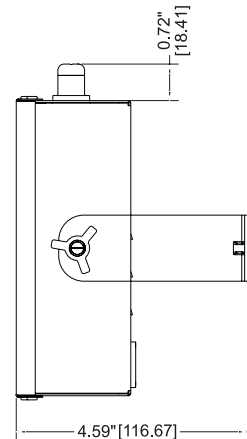
Wall Mount
